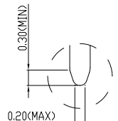
VIEW A SCALE 5:1
