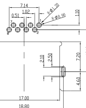
RECOMMENDED PCB LAYOUT TOP VIEW: TOL:±0.05mm
