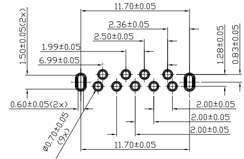
REFERENCE PCB LAYOUT
