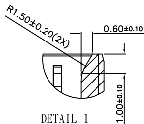
DETAIL 1 SCALE 8 : 1
