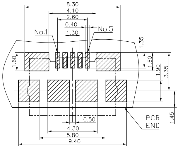
PCB LAYOUT *General tolerance is ±0.05mm.
