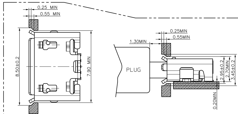
RECOMMENDED PANEL CUTOUT MATED WITH CORRESPONDING PLUG
