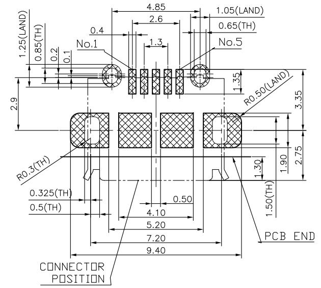
PCB LAYOUT *General tolerance is ±0.05mm.
